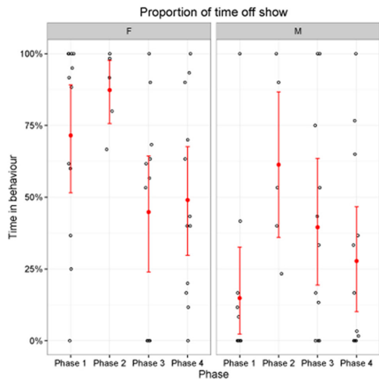
Figure 1. Proportion of time off-show by phase. Individual observations are shown as black points (horizontally jittered to reduce over-plotting). Mean and bootstrapped 95% confidence intervals for each phase/behaviour are in red.
